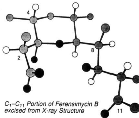
Figure 3. \text{C}_1 - \text{C}_{11} portion of ferensimycin B excised from X-ray structure.
