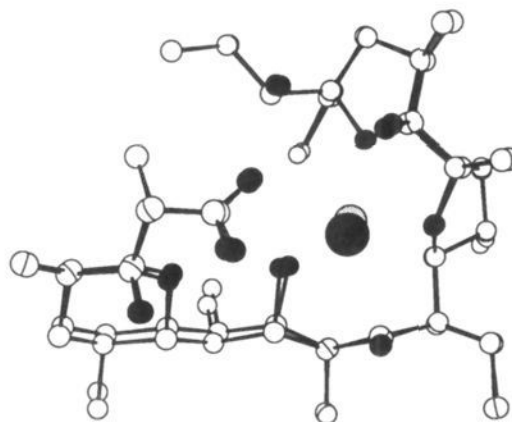
Figure 2. Superposition of ferensimycin-thallium(I) and lysocecellin-silver(I) complexes.
